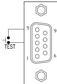
Figure 1.0: Slaughter Model 1305 Signal Input Connector
