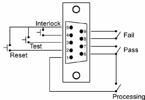
Figure 3.0: Slaughter Model 2550 Remote I/O Connector
