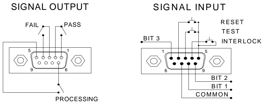
Figure 4.0: Slaughter Model 4320 Remote I/O Connectors
