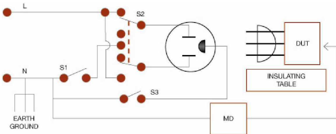
Figure 1: LLT Schematic
